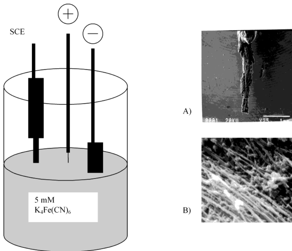
Figure 1. Schematic showing the electrochemical cell used in the experiments for the K_4Fe(CN)_6 reaction. (A) Shows the close-up view of the tip of the anode assembly, which is the nanotube bundle. (B) Shows the microstructure of a small area on the porous nanotube electrode; the fibers seen in this image correspond to individual multiwalled nanotubes. There is a range of sizes for the nanotubes (2–25 nm diameter and up to several microns). Closed nanosize polyhedral particles of graphitic carbon can also be seen along with tubes, but the surface structure of the former is essentially the same, exposing only the graphite basal planes.
