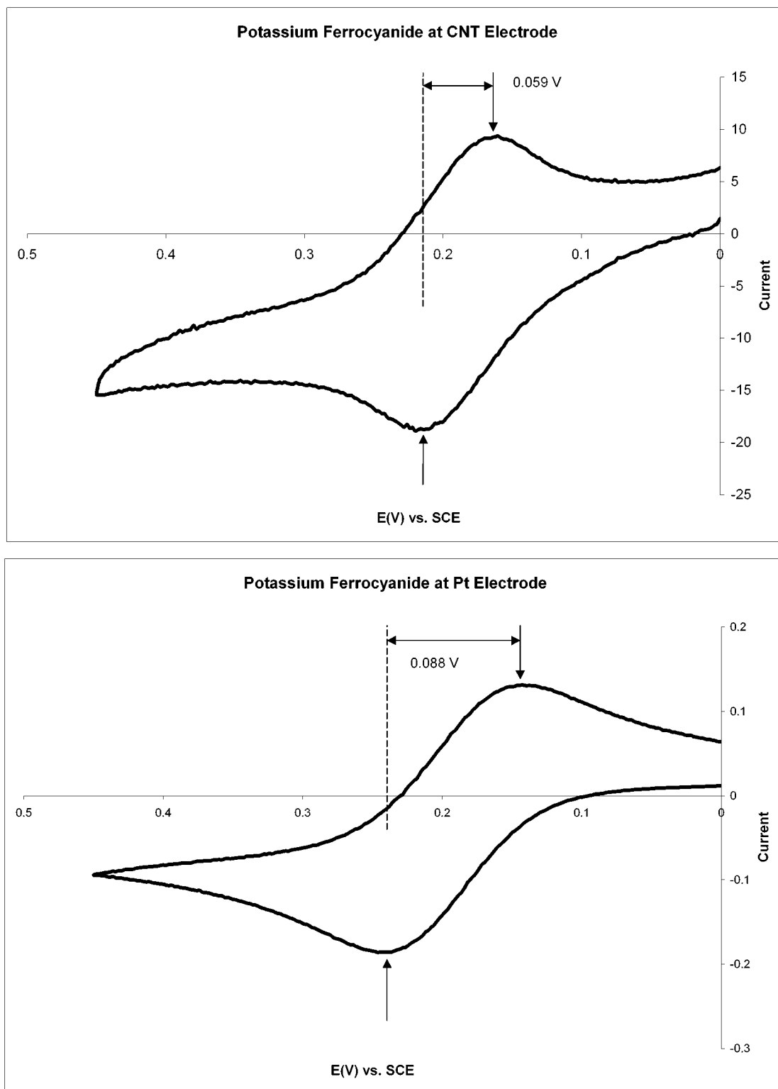
Figure 2. Cyclic voltammetric curves of 5 mM K_4Fe(CN)_6 on a Pt electrode (bottom) and a carbon nanotube microbundle electrode (top) recorded using a 273 PAR Potentiostat/ Galvanostat. A Pt foil is used as the counter electrode and saturated calomel electrode (SCE) as the reference electrode. The anodic peak potential is situated at E_{pa} = 0.220 V and the complementary cathodic peak at E_{pc} = 0.161 V. The peak potentials did not change with increasing sweep rate up to a high sweep rate of 1 V/s. The current on the Y-axis is plotted in units of microamps. Notice the big difference in the background currents for the two electrodes. The apparent electrode areas (calculated from the outer dimensions of the electrodes) of Pt and the nanotube electrodes used in this study are 0.14 \text{ cm}^2 and 0.009 \text{ cm}^2 respectively; the real surface area available for electrochemistry for the nanotube electrode could be far greater due to the high porosity of the electrode.
